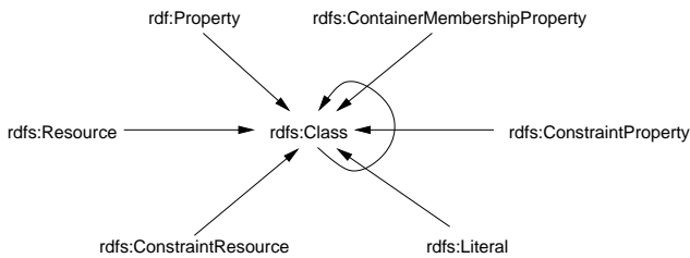
Figure 3. The instance-of relationships of modeling primitives in RDFS.
