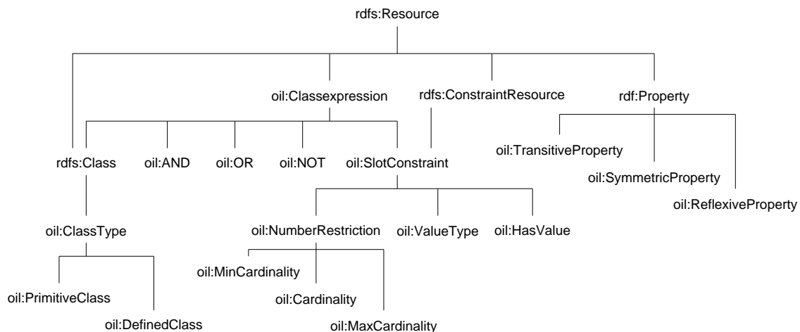
Figure 5. The OIL extensions to RDFS in the subsumption hierarchy.
