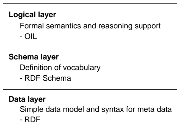
Figure 1. The three-layered architecture of the Semantic Web
