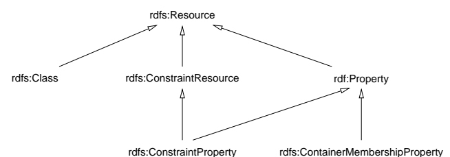
Figure 2. The subclass-of hierarchy of modeling primitives in RDFS.
